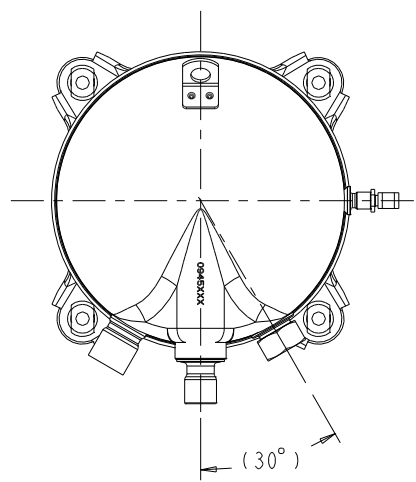
SIGHTGLASS LAYOUT T-BOX REMOVED
