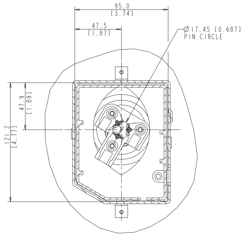
T-BOX LAYOUT STANDARD SECTION A-A SCALE 1:1
