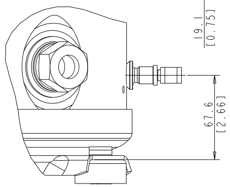
DETAIL VALVE SCALE 3:4
